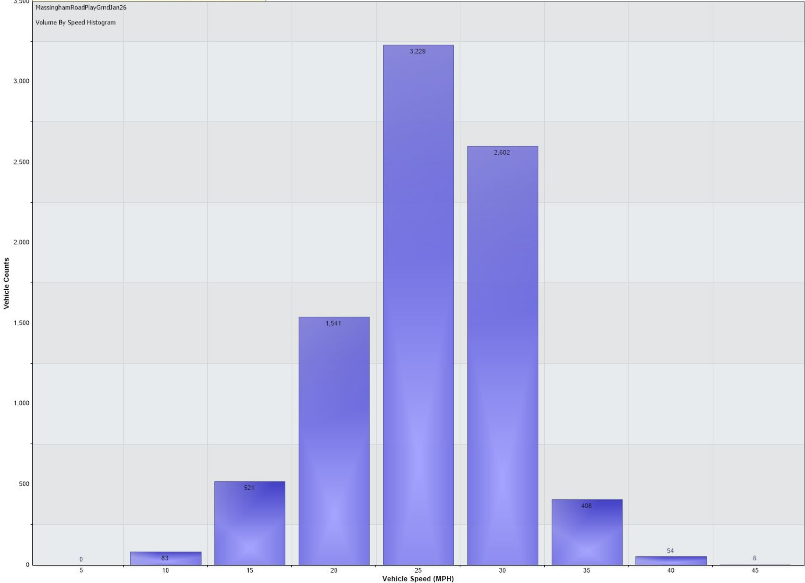
Vehicle Counts Vs. Speed [MassinghamRoadPlayGrndJan26: Incoming]
